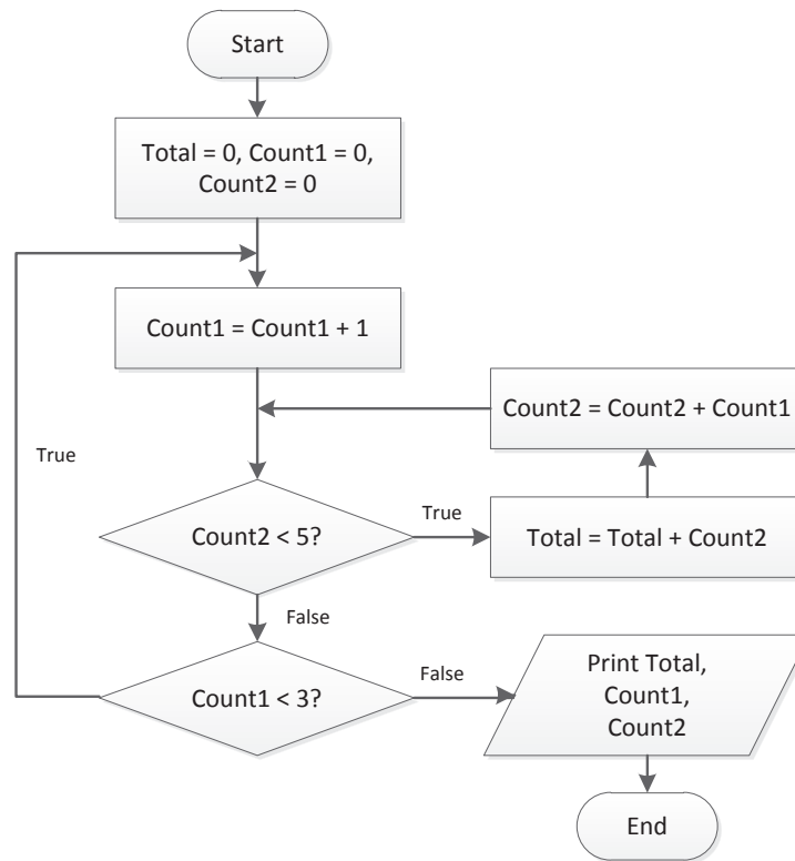
Figure 1: Flowchart
