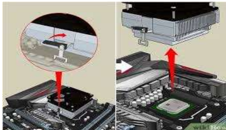
Figure 60: Step to install heat sink
