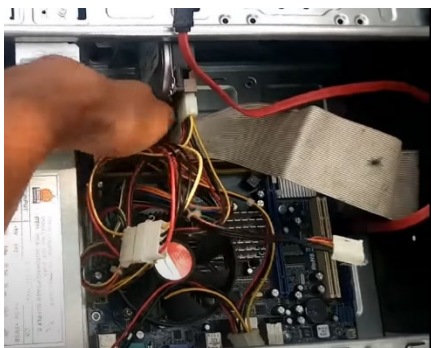
Figure 27. Connect power cable to motherboard, hard disk, graphic cards and accessories. From How to Make or Assemble Desktop CPU Step by Step At Home | How to Build a Computer with used Parts .
