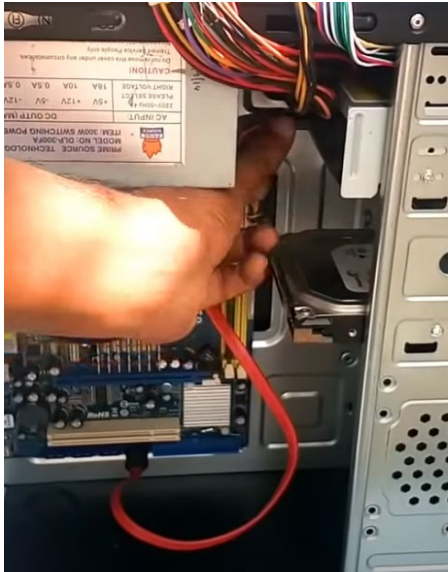
Figure 25. Connect SATA cable to motherboard and CD ROM. From How to Make or Assemble Desktop CPU Step by Step At Home | How to Build a Computer with used Parts .
