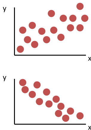
Linear relationships
