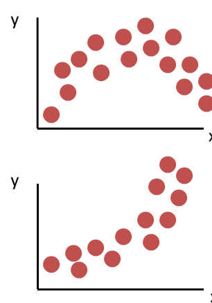
Curvilinear relationships
