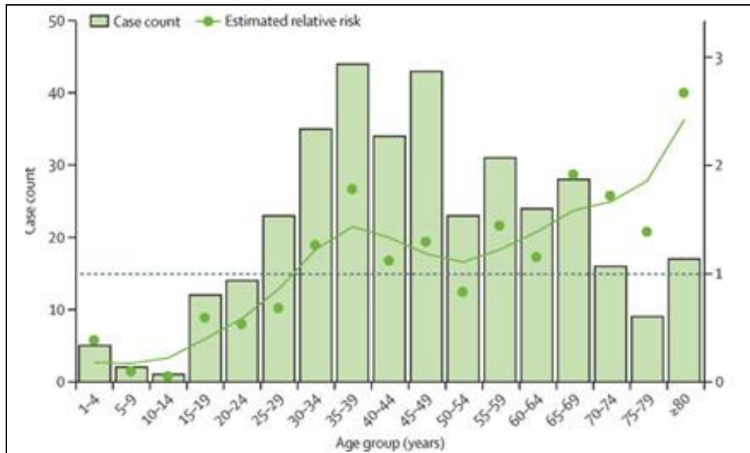
Figure 1: Age Distribution of COVID-19 Patients in China
