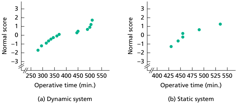
FIGURE 10.5 Normal probability plots of the sample data for the (a) dynamic system and (b) static system
