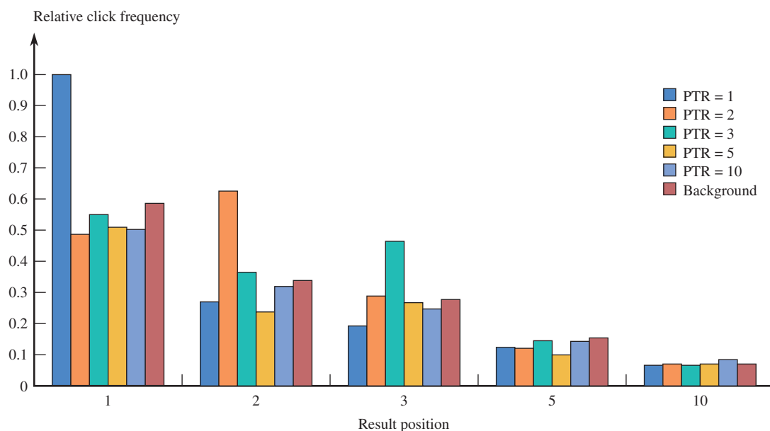
FIGURE 3.37 Comparative bar graph for click frequency data.
