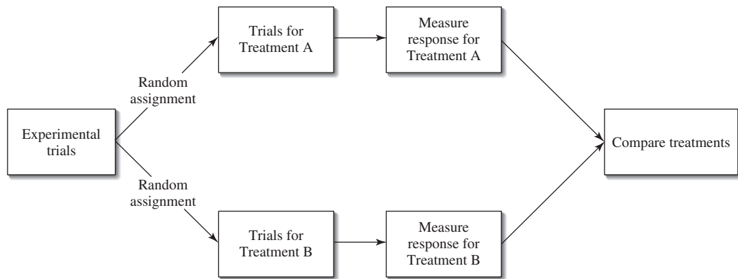
FIGURE 2.6 Diagram of an experiment with random assignment of treatments to trials.
