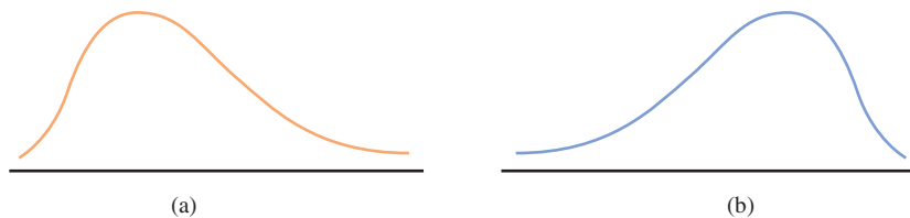
FIGURE 3.27 Two examples of skewed smoothed histograms: (a) positive skew; (b) negative skew.
