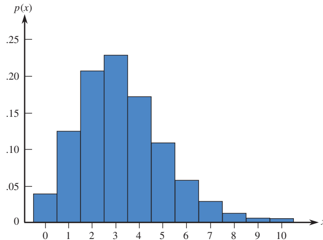
FIGURE 7.4 Probability histogram for the distribution of the number of minor paint blemishes on a randomly selected car.
