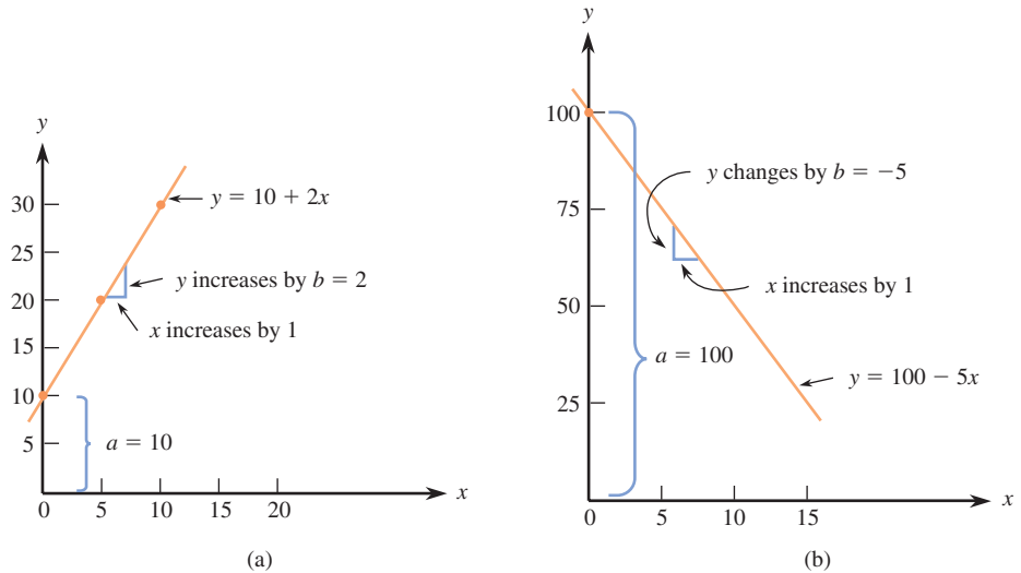
FIGURE 5.7 Graphs of two lines: (a) slope b = 2 , intercept a = 10 ; (b) slope b = -5 , intercept a = 100 .
