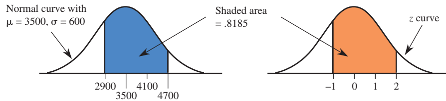
FIGURE 7.29 P(2900 < x < 4700) and corresponding z curve area for the birth weight distribution of Example 7.27.
