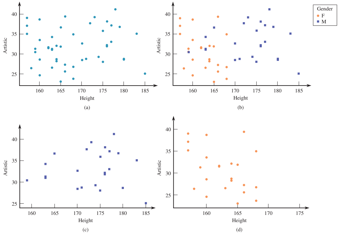
FIGURE 3.33 Scatterplots for the data of Example 3.20: (a) scatterplot of data; (b) scatterplot of data with observations for males and females distinguished by color; (c) scatterplot for male skaters; (d) scatterplot for female skaters.
