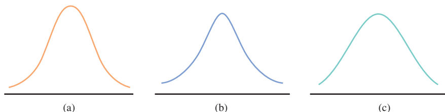
FIGURE 3.28 Three examples of bell-shaped histograms: (a) normal; (b) heavy-tailed; (c) light-tailed.
