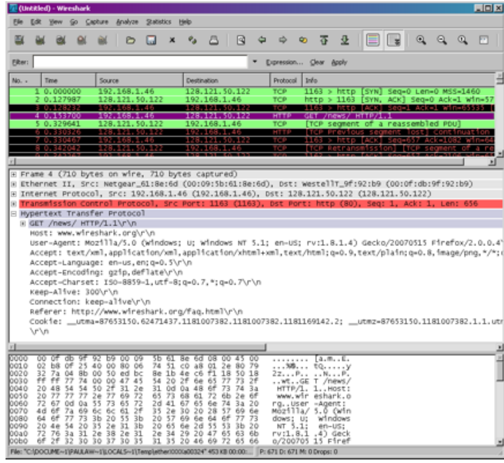
Figure A.3: Wireshark Graphical User Interface, during packet capture and
