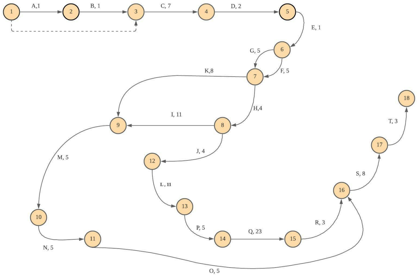
Figure 4: Pert Diagram
