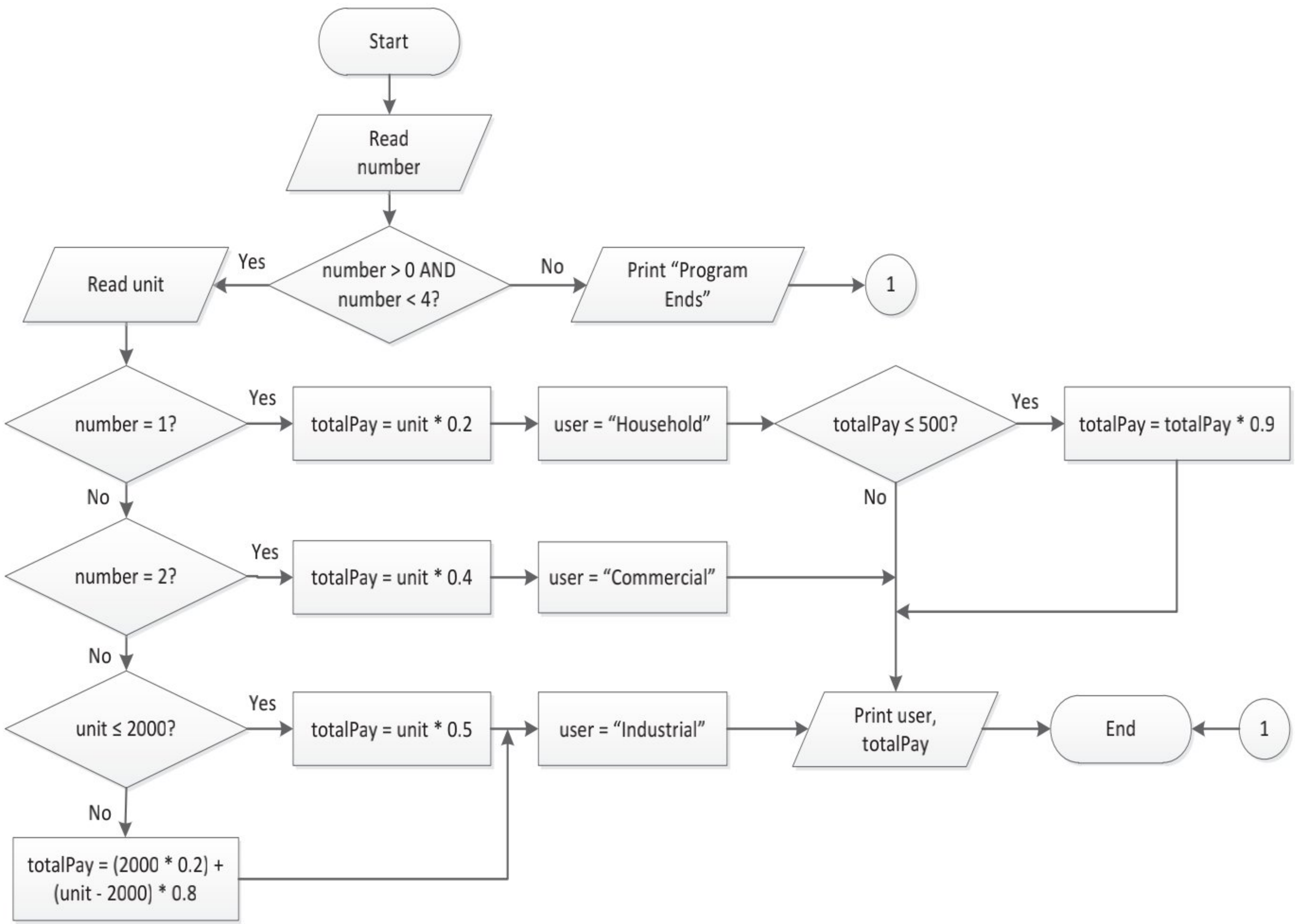
Figure 7: Flowchart
