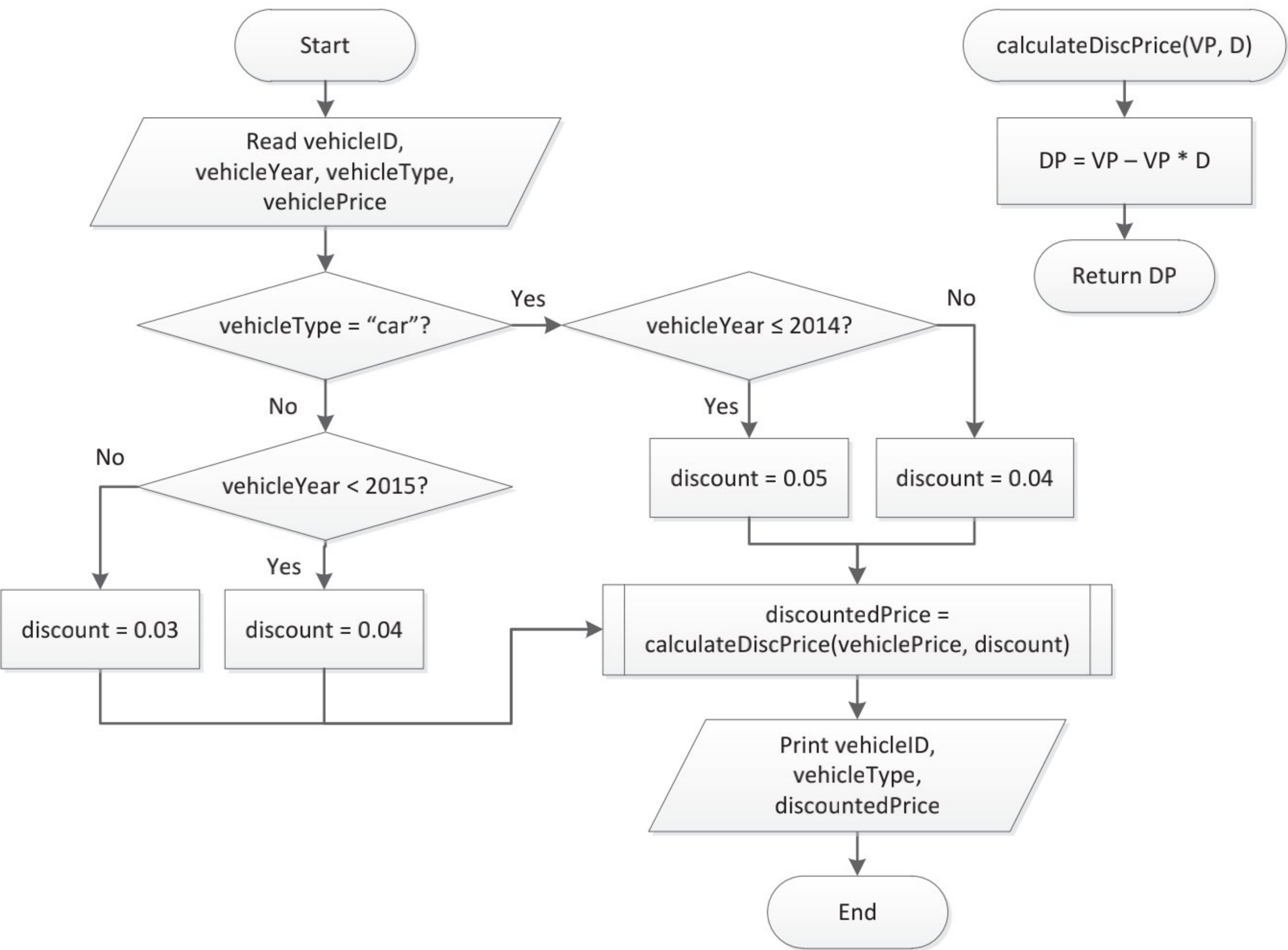
Figure 4: Flowchart
