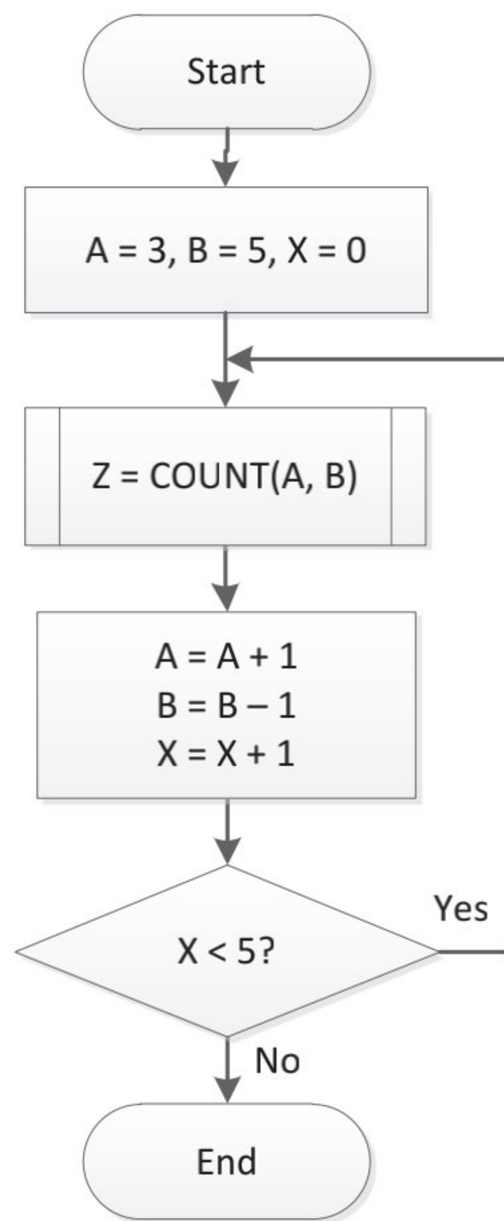
Figure 5: Flowchart 1
