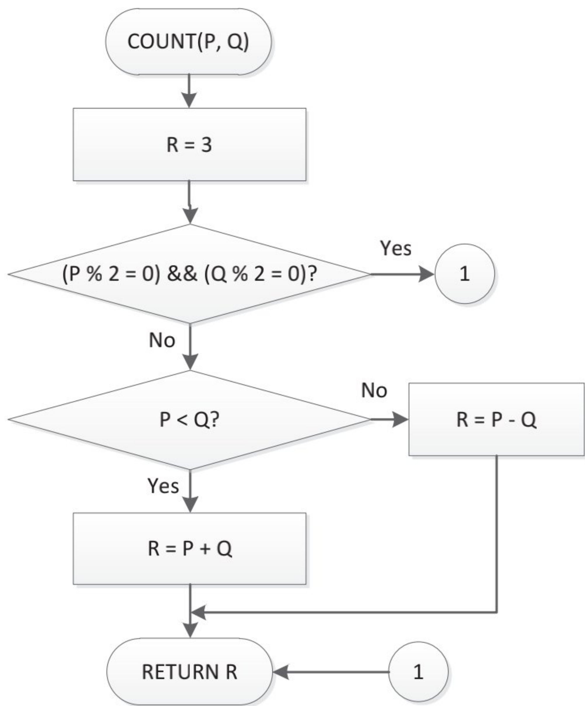
Figure 6: Flowchart 2
