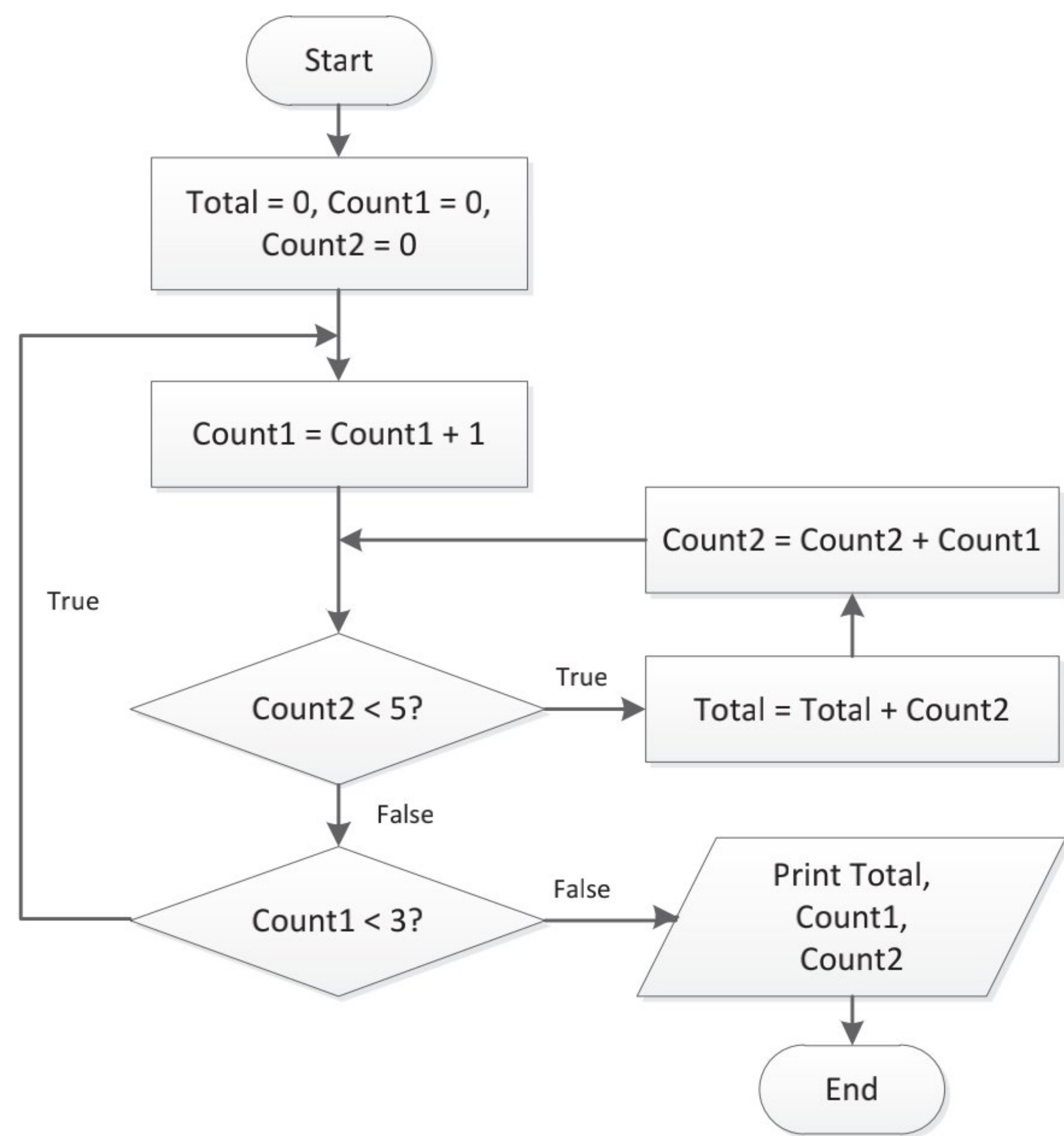
Figure 1: Flowchart
