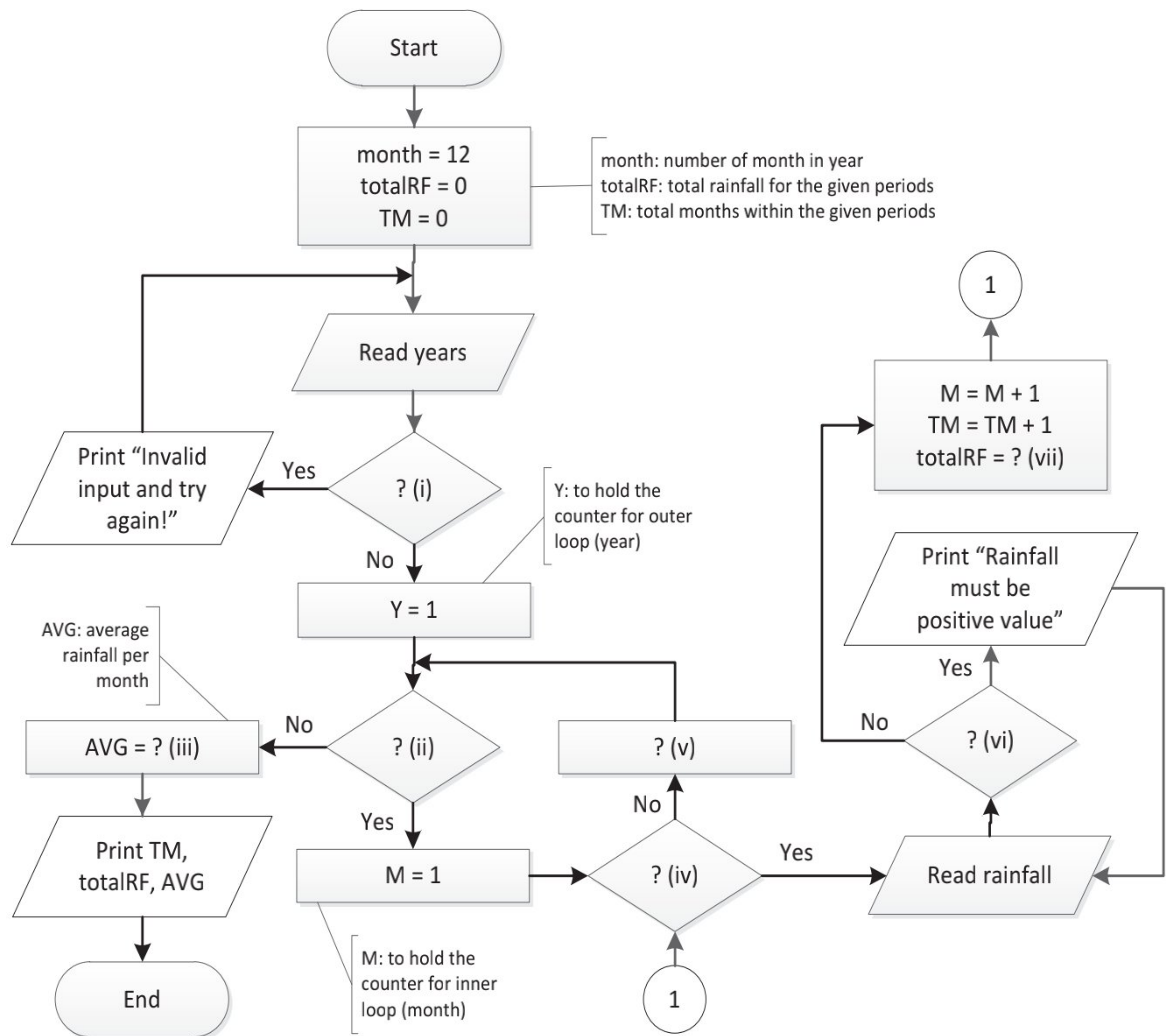
Figure 3: Flowchart
