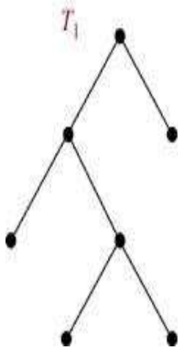
full binary tree
