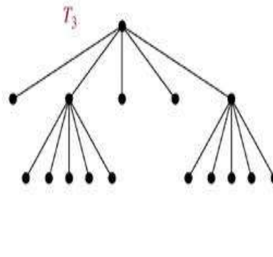
full 5-ary tree
