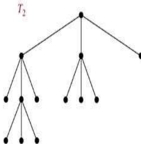
full 3-ary tree
